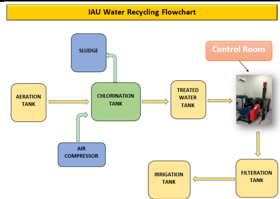
Water Recycling Flow Chart in IAU
